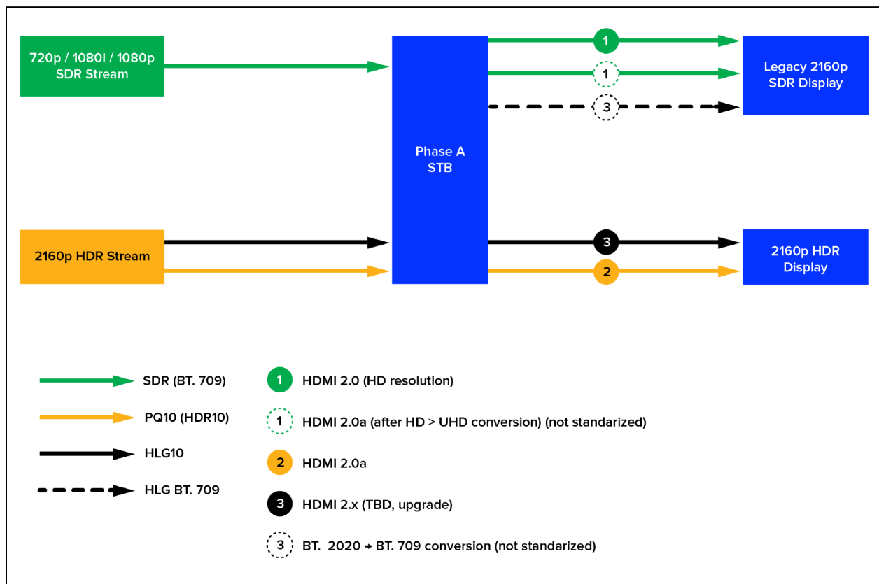
Figure 29 Spatial Resolution Up-conversion of Legacy Services
