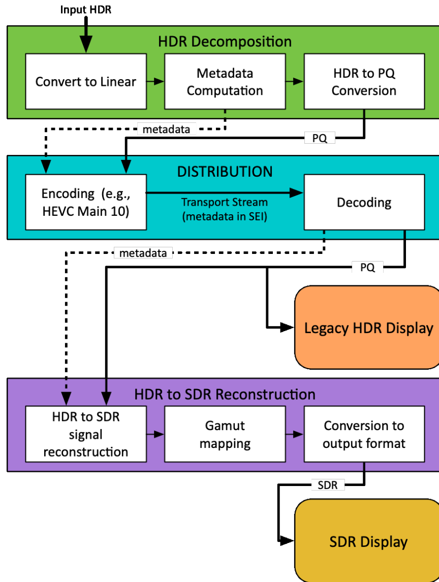
Figure 45 SL-HDR2 processing, distribution, reconstruction, and SDR presentation
