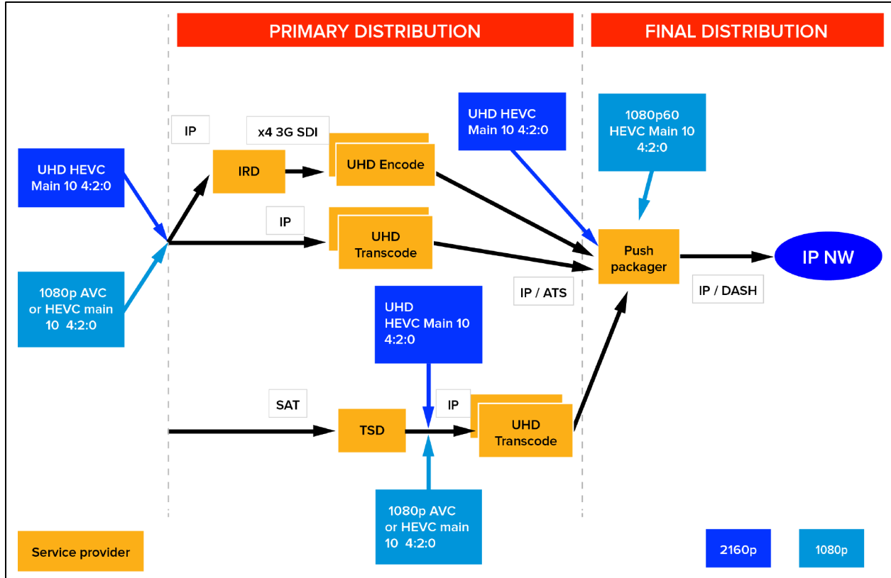
Figure 25 Primary Distribution to an OTT Provider
