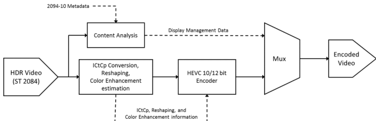
Figure 30 Encoder functional block diagram
