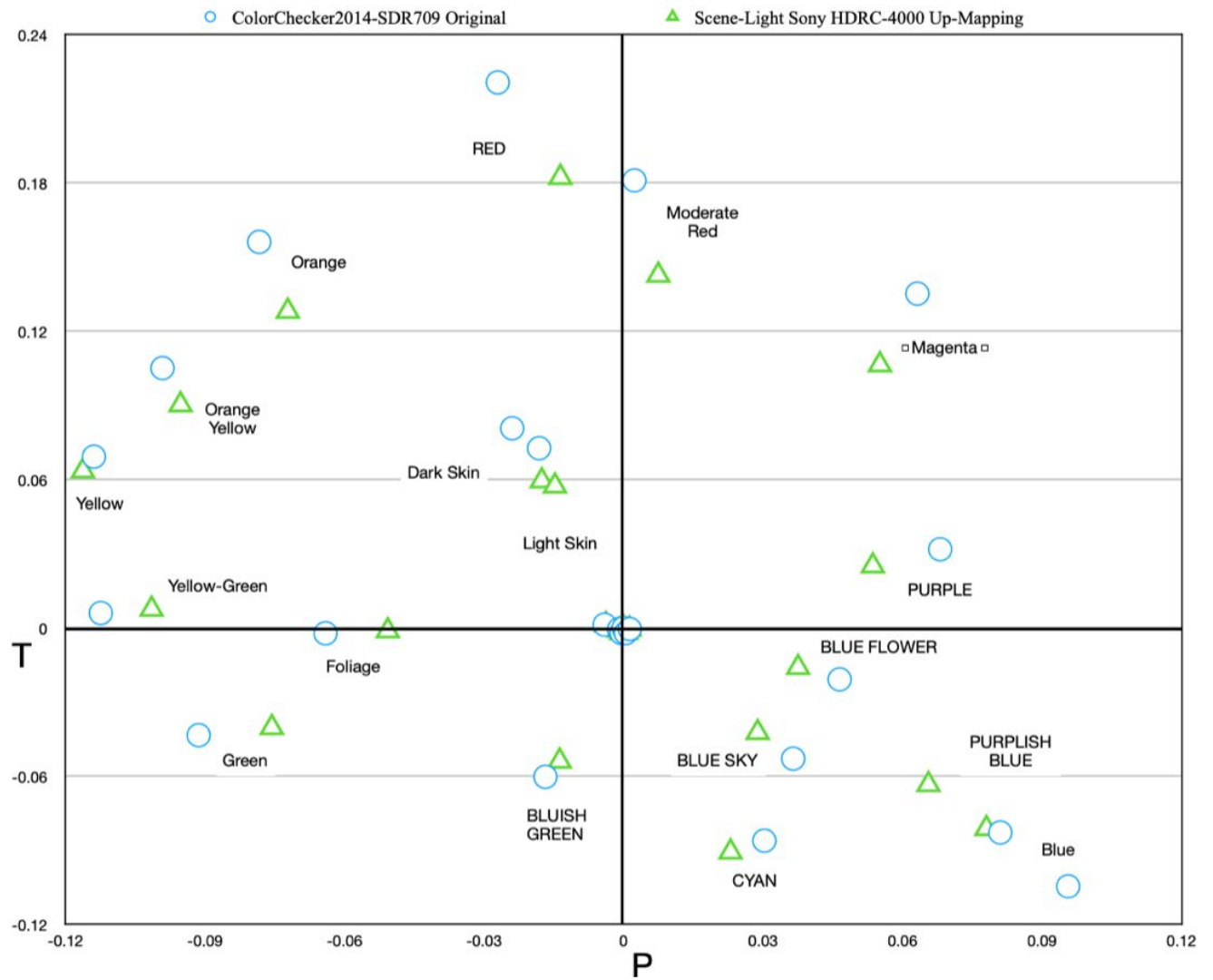
Figure 15 Scene Light Conversion Accuracy, SDR to HLG
