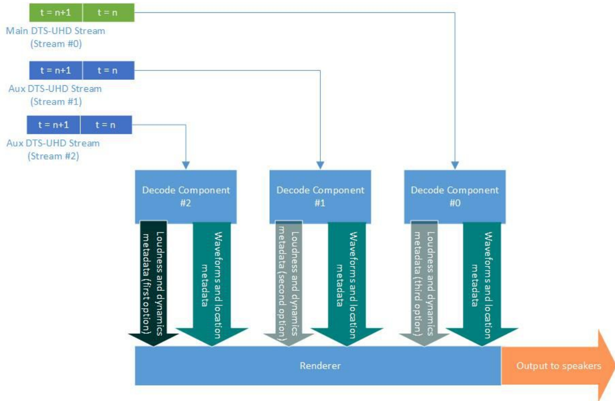
Figure 77 Example of multi-stream decoding
