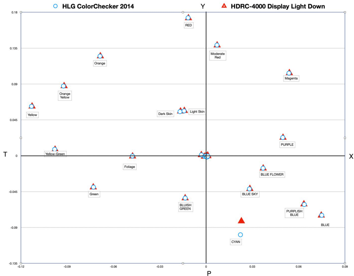
Figure 17 Down-Mapping HLG to SDR Color Accuracy
