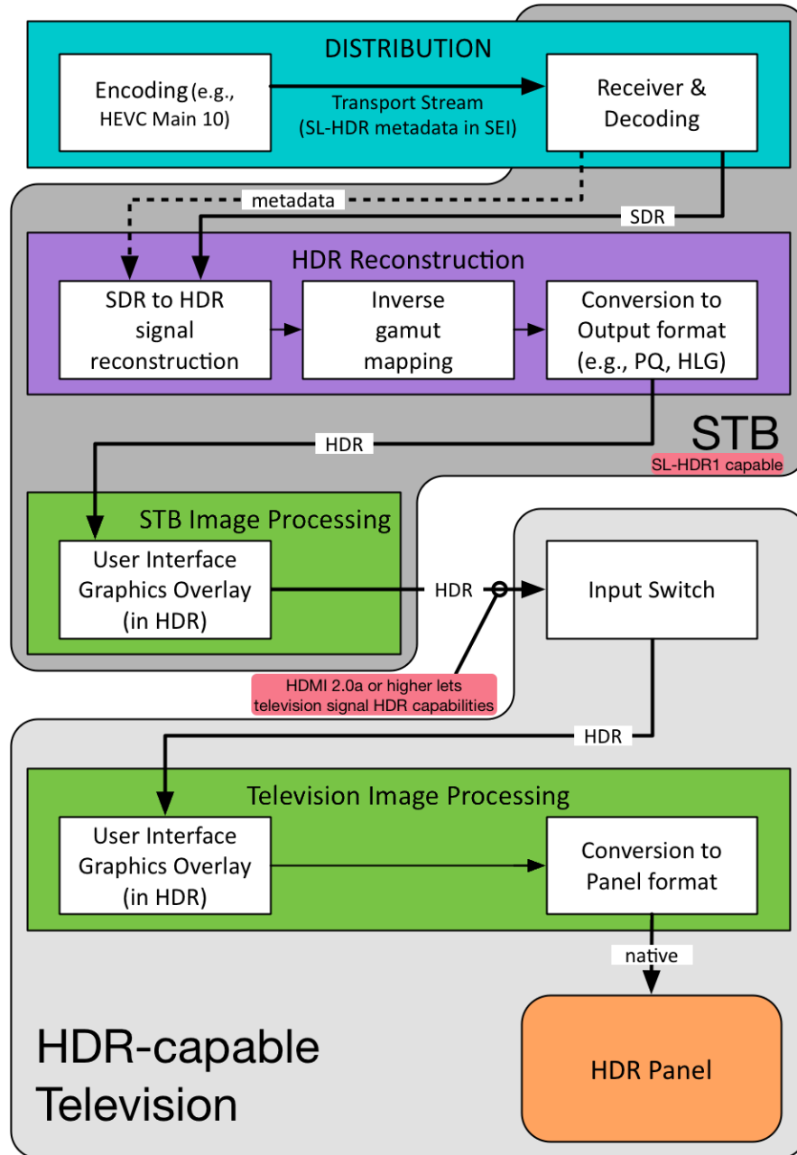
Figure 39 STB processing of SL-HDR signals for an HDR-capable television
