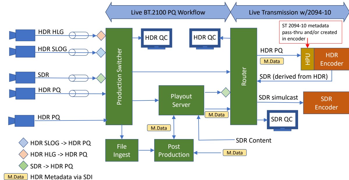
Figure 35 HDR broadcast production facility with BT.2100 PQ workflow- SDI metadata
