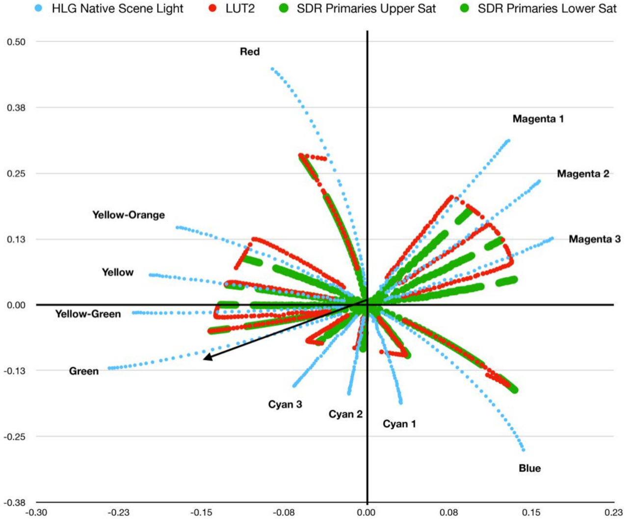
Figure 20 LUT2 Conversion from HLG to SDR
