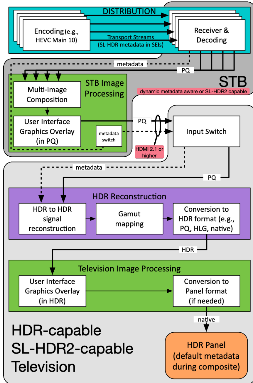
Figure 49 Multiple SL-HDR channels received and composited in HDR by an STB
