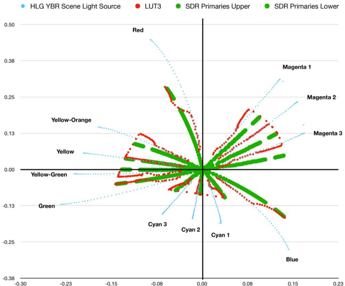
Figure 21 LUT 3 Conversion from HLG to SDR
