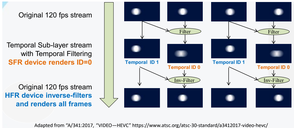
Figure 53 ATSC 3.0 temporal filtering for HFR backward compatibility
