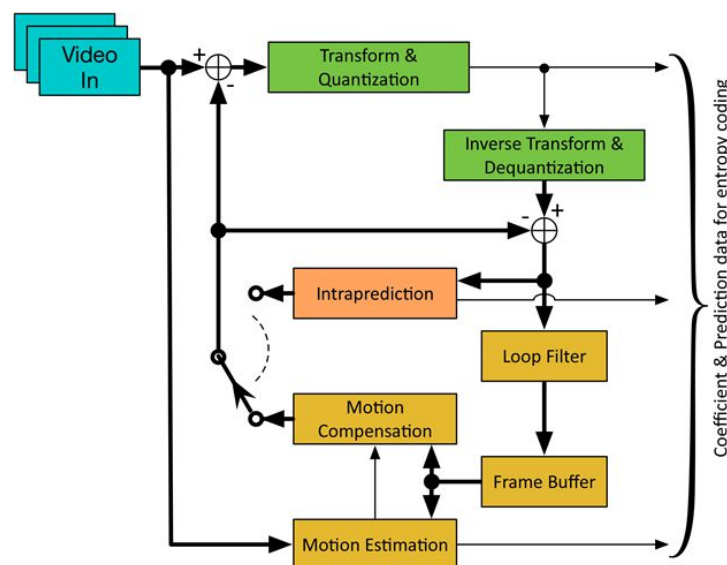
Figure 92 AVS2 coding framework
