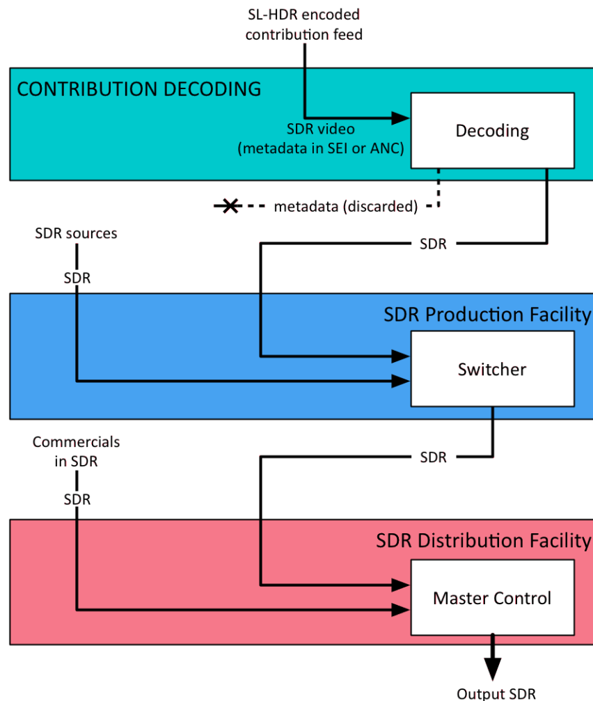
Figure 43 SL-HDR as a contribution feed to an SDR facility
