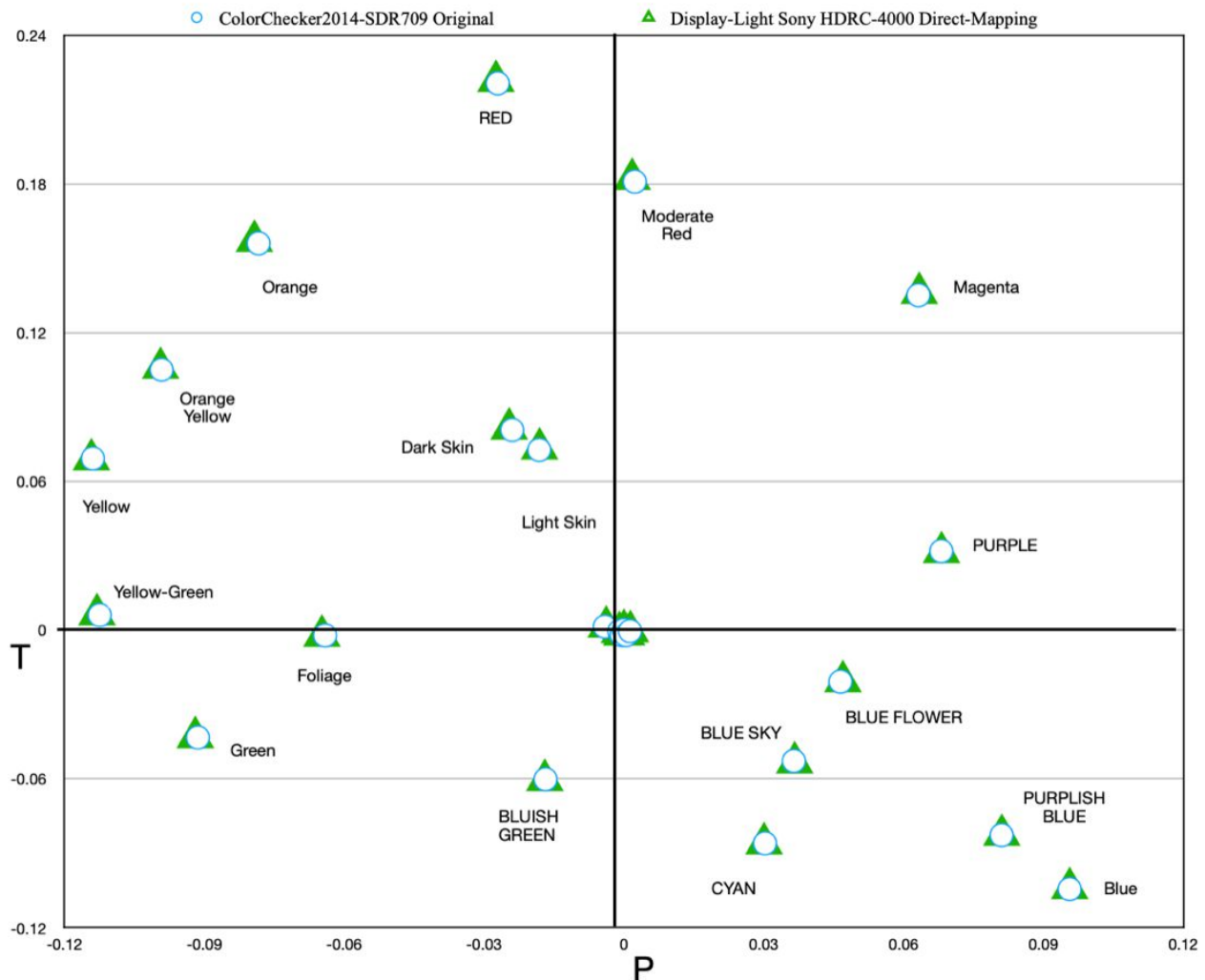
Figure 16 Display Light Conversion Accuracy, SDR to HLG
