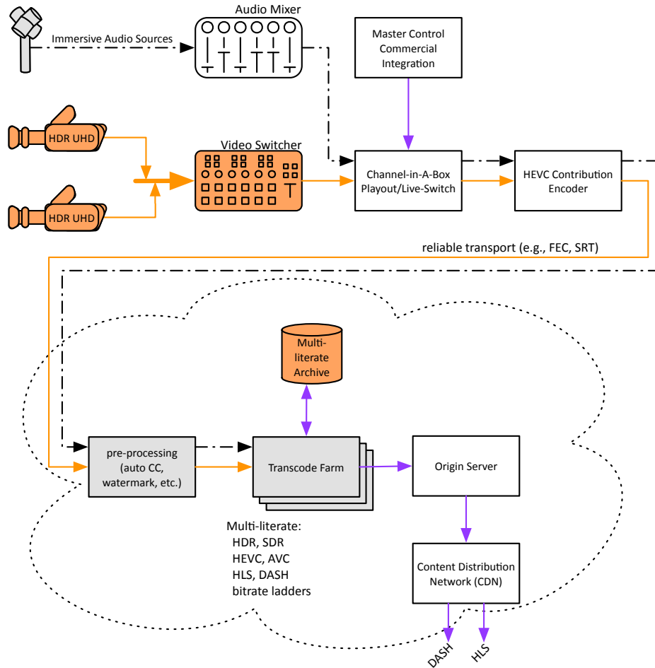
Figure 26 Live Event Streaming over OTT Workflow
