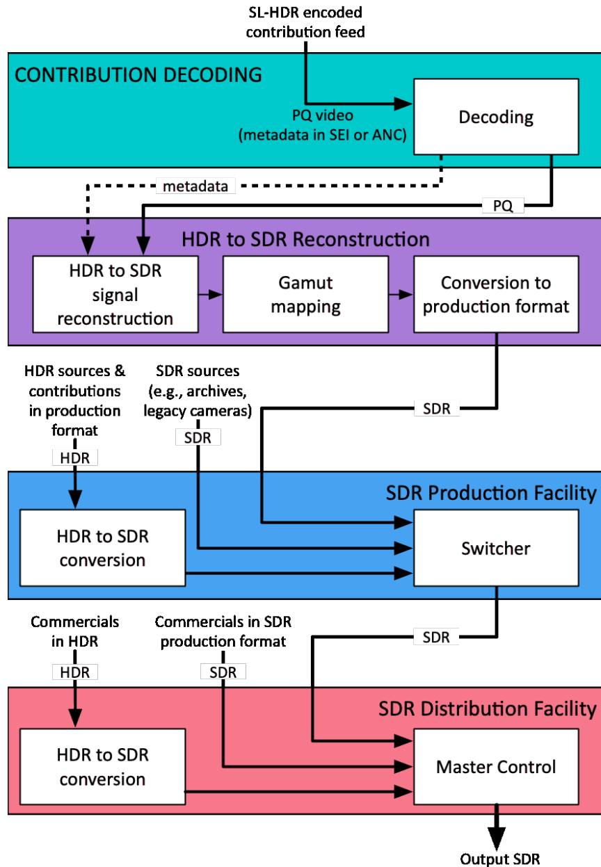
Figure 51 SL-HDR as a contribution feed to an SDR facility
