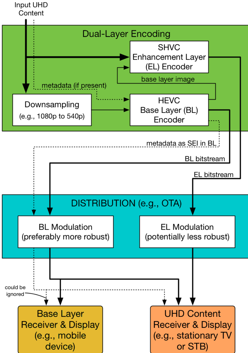
Figure 36 Example dual-layer encoding and distribution
