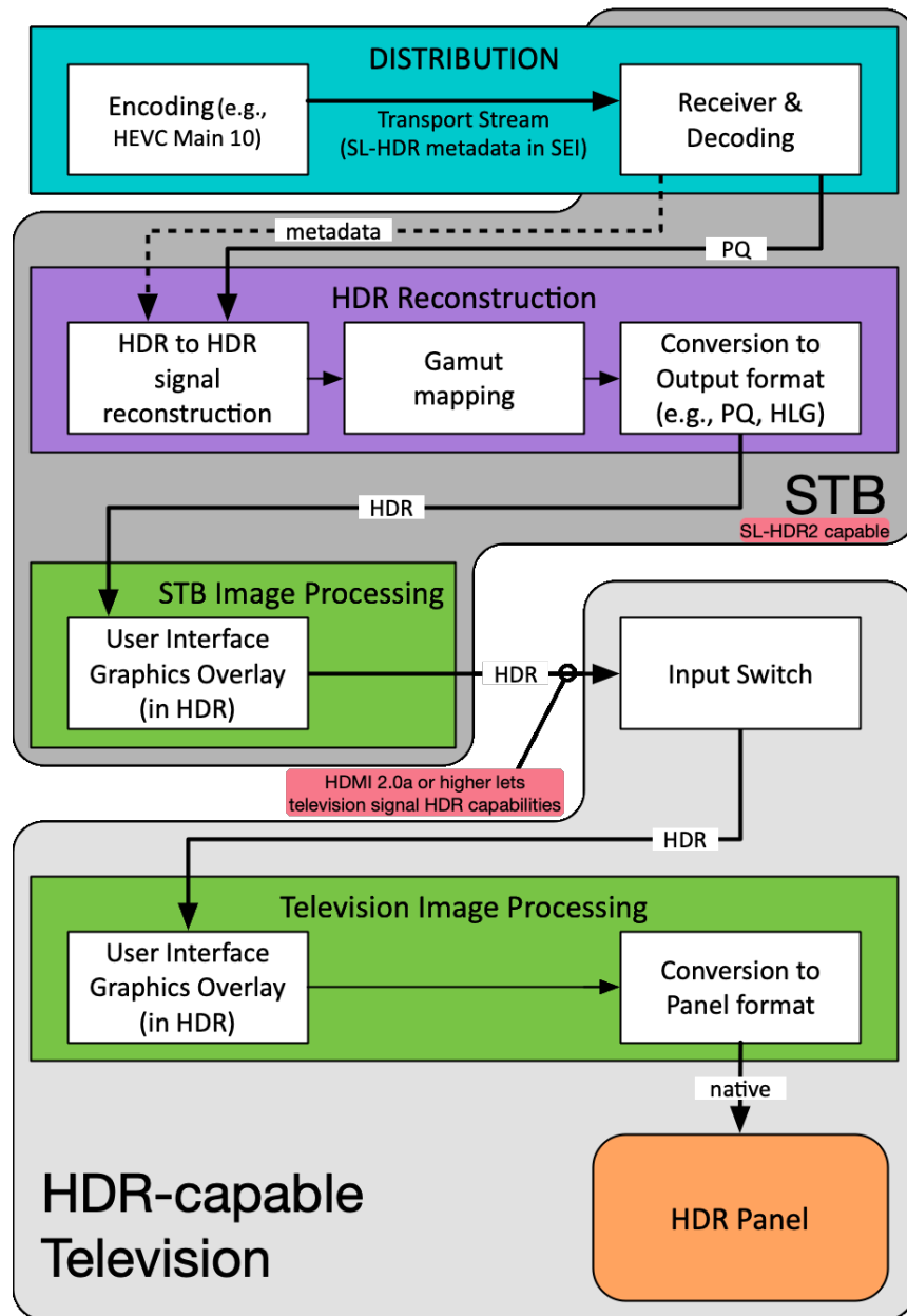
Figure 47 STB processing of SL-HDR signals for an HDR-capable television
