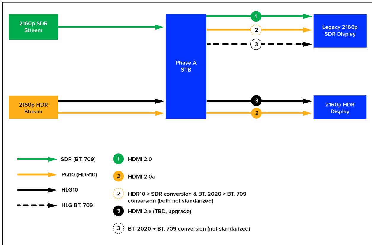
Figure 28 Down-conversion at the STB
