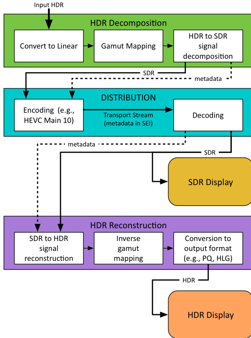
Figure 37 SL-HDR processing, distribution, reconstruction, and presentation
