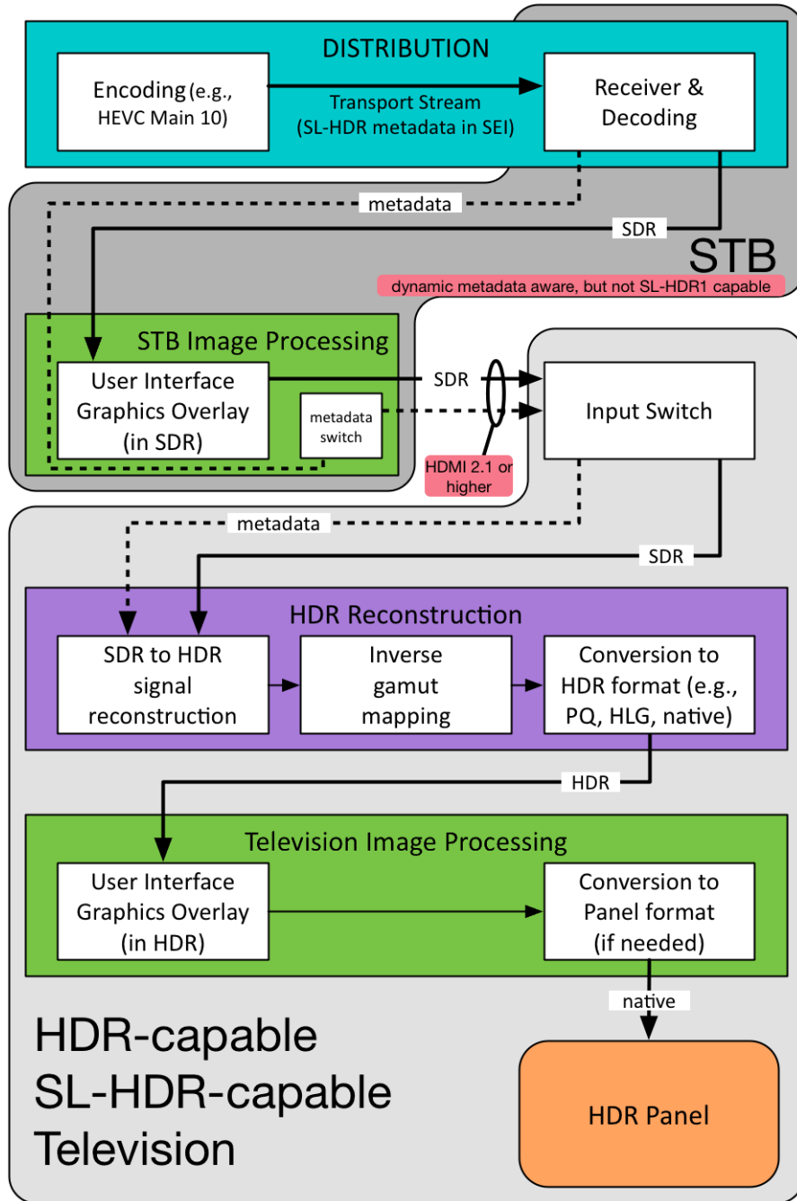
Figure 40 STB passing SL-HDR to an SL-HDR1 capable television
