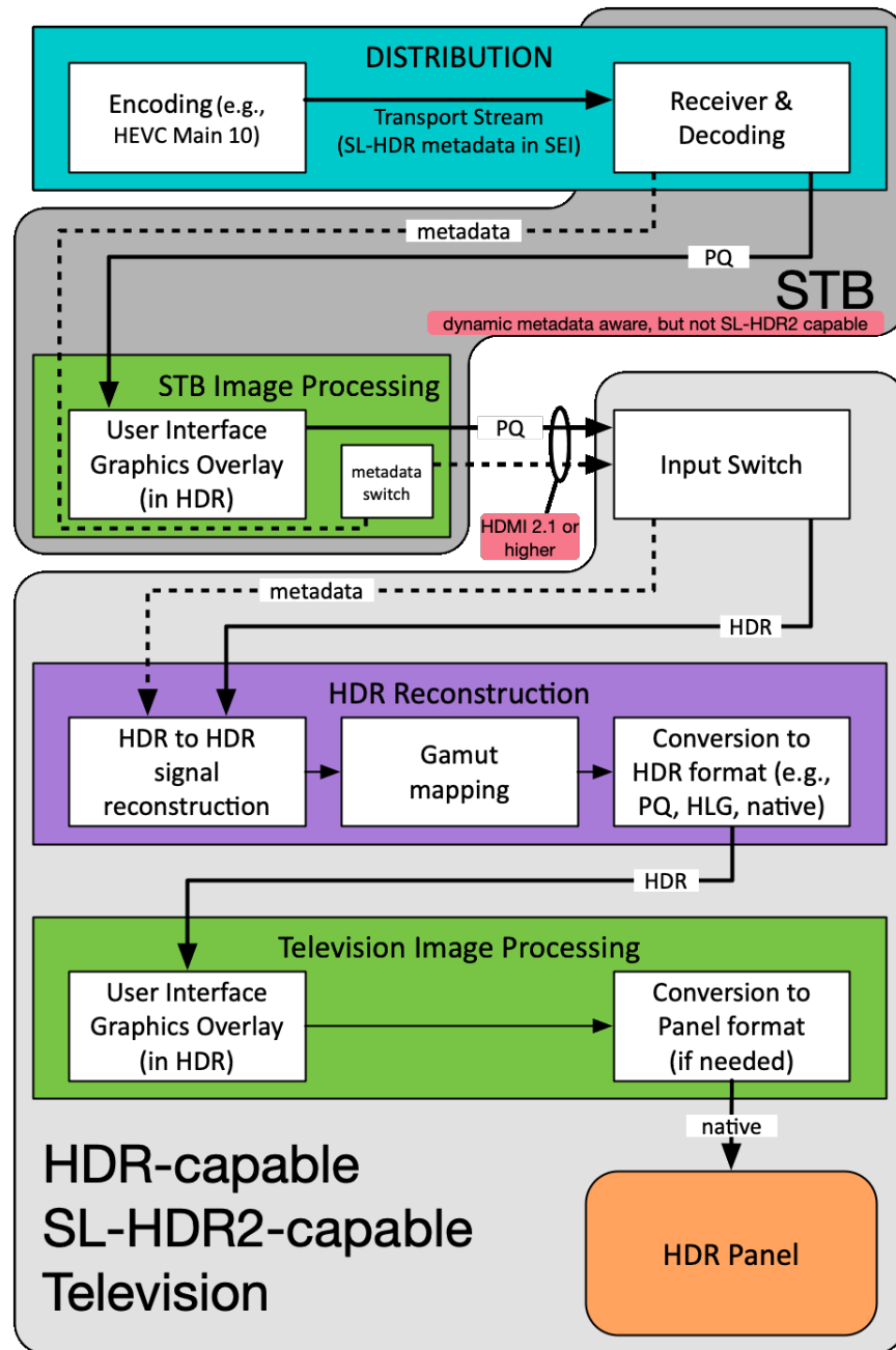
Figure 48 STB passing SL-HDR to an SL-HDR2 capable television
