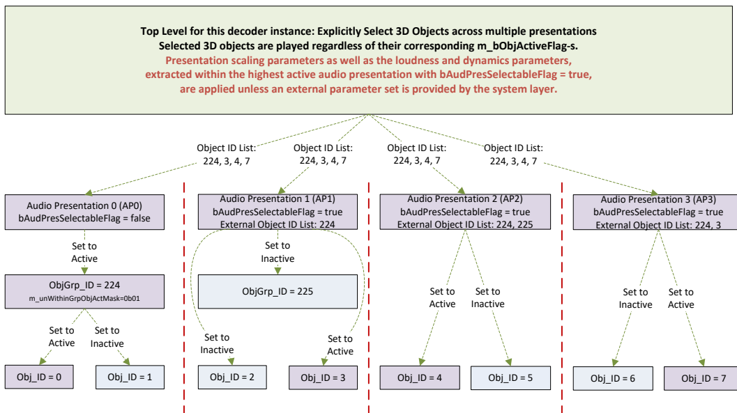
Figure 76 Example of Selecting Desired Objects to Play Within a Single Stream
