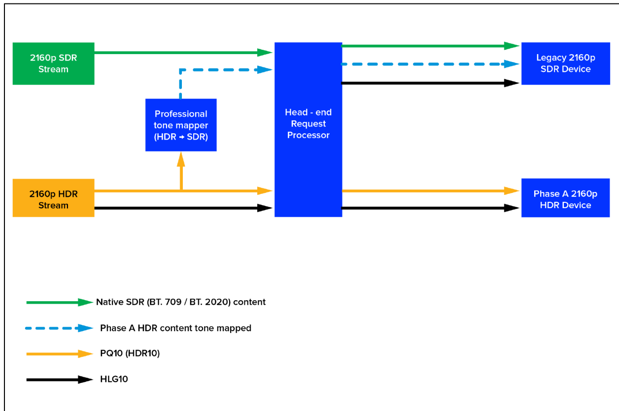
Figure 27 Down-conversion at the Headend
