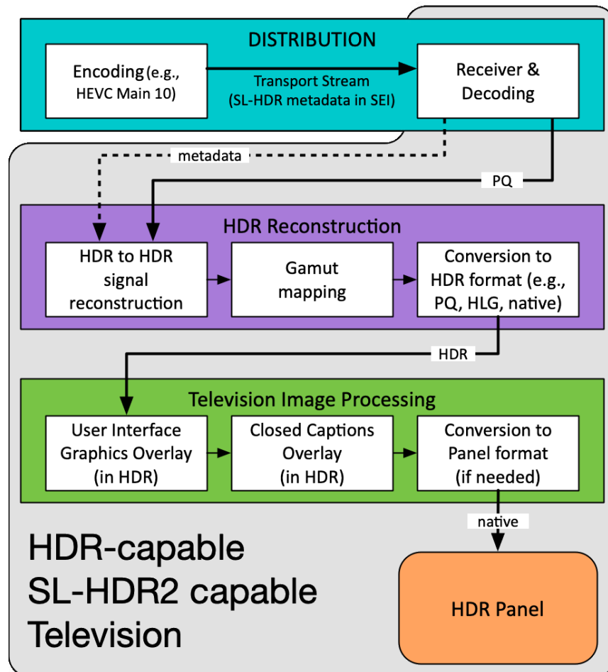
Figure 46 Direct reception of SL-HDR signal by an SL-HDR2 capable television
