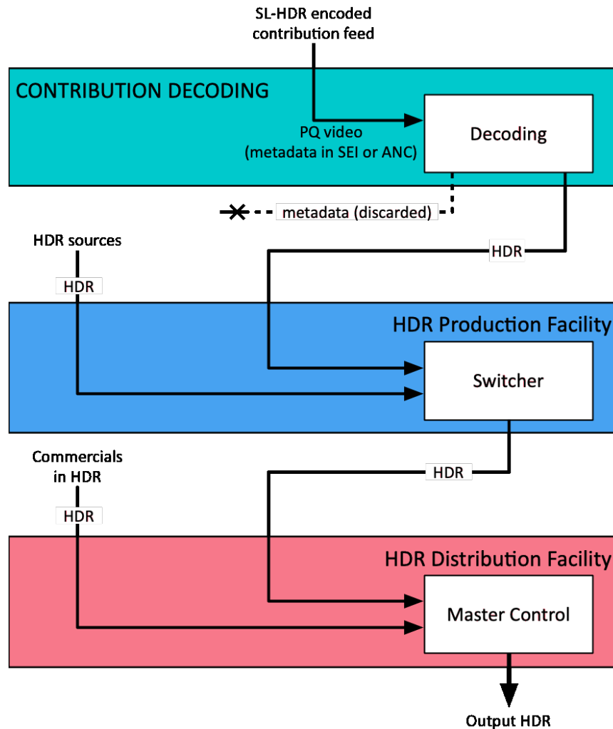
Figure 50 SL-HDR as a contribution feed to an HDR facility
