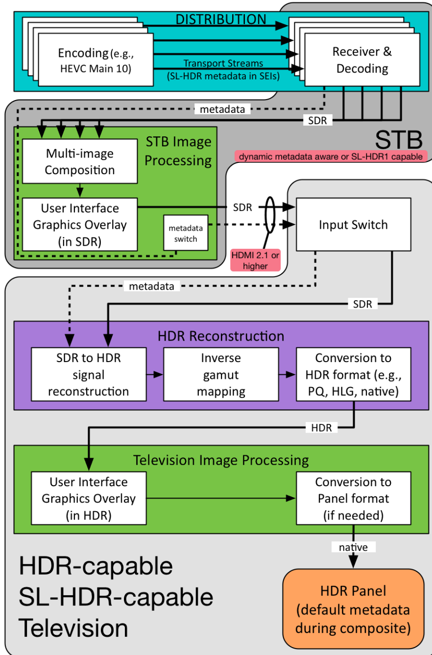
Figure 41 Multiple SL-HDR channels received and composited in SDR by an STB
