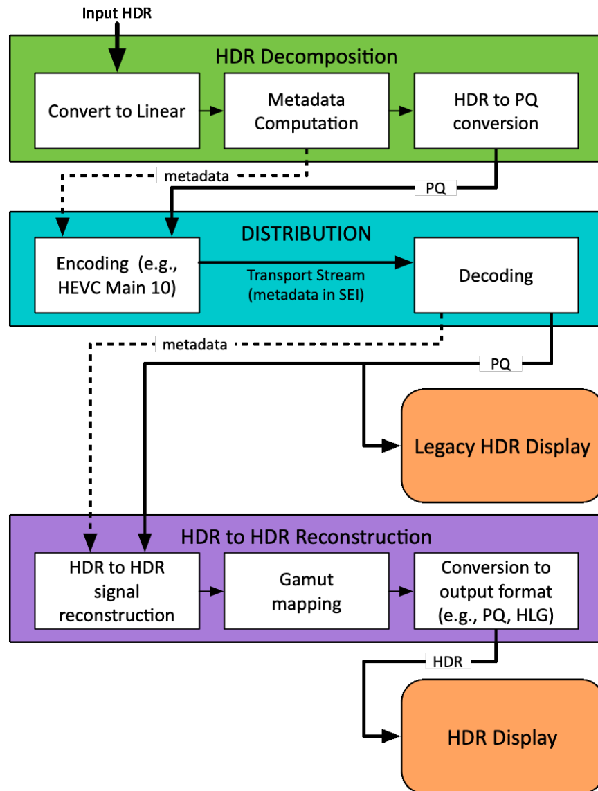
Figure 44 SL-HDR2 processing, distribution, reconstruction, for HDR presentation
