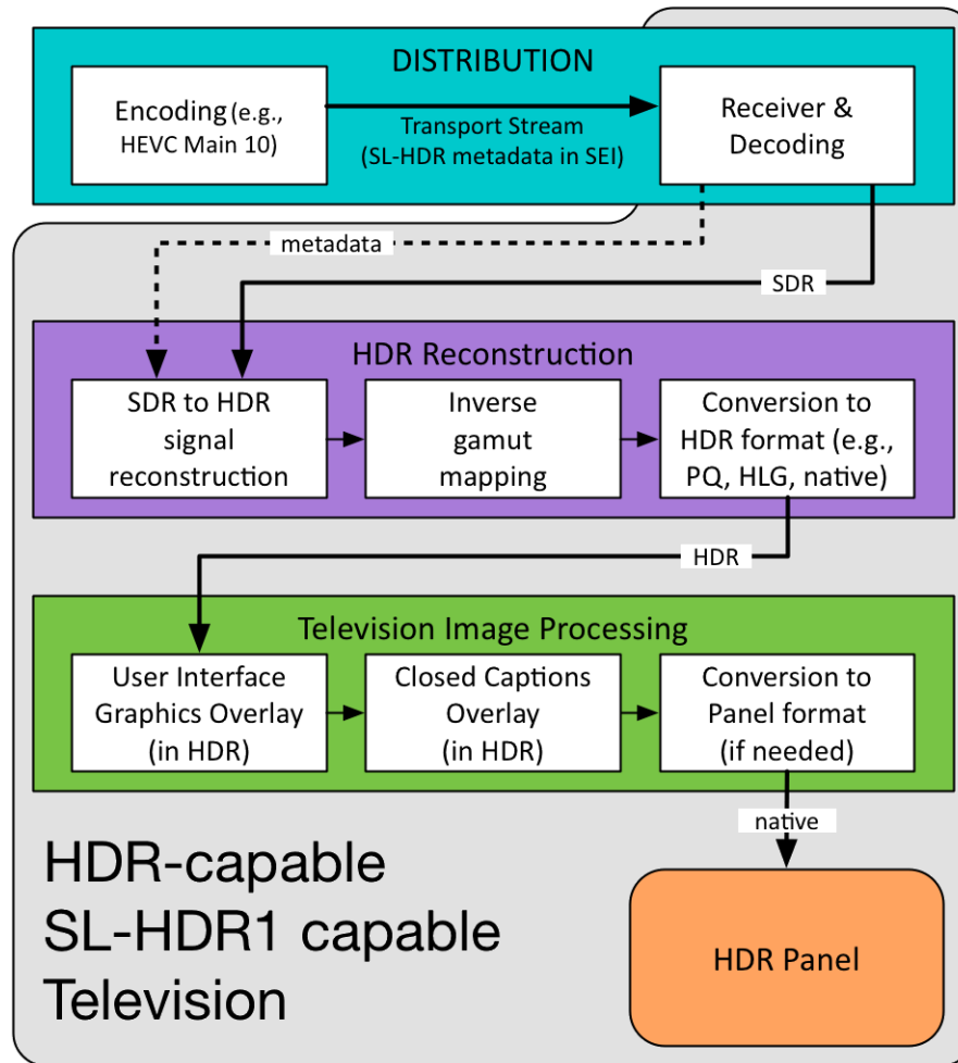
Figure 38 Direct reception of SL-HDR signal by an SL-HDR1 capable television
