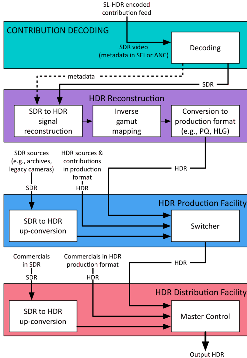
Figure 42 SL-HDR as a contribution feed to an HDR facility
