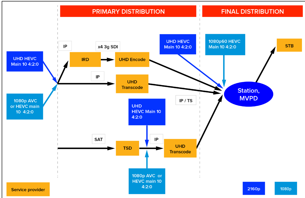
Figure 24 Primary Distribution to an MVPD or Station
