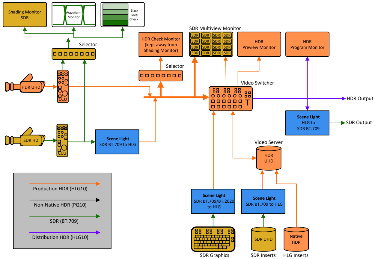
Figure 88 Sky/BBC Royal Wedding and Major Tennis Tournament Workflow
