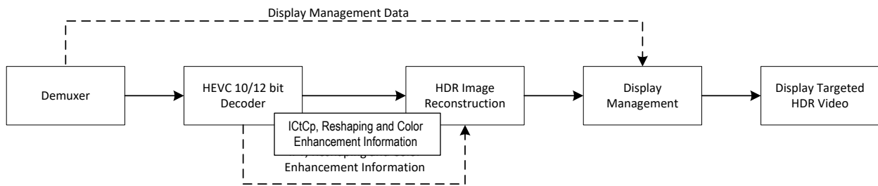
Figure 31 Decoder function block diagram
