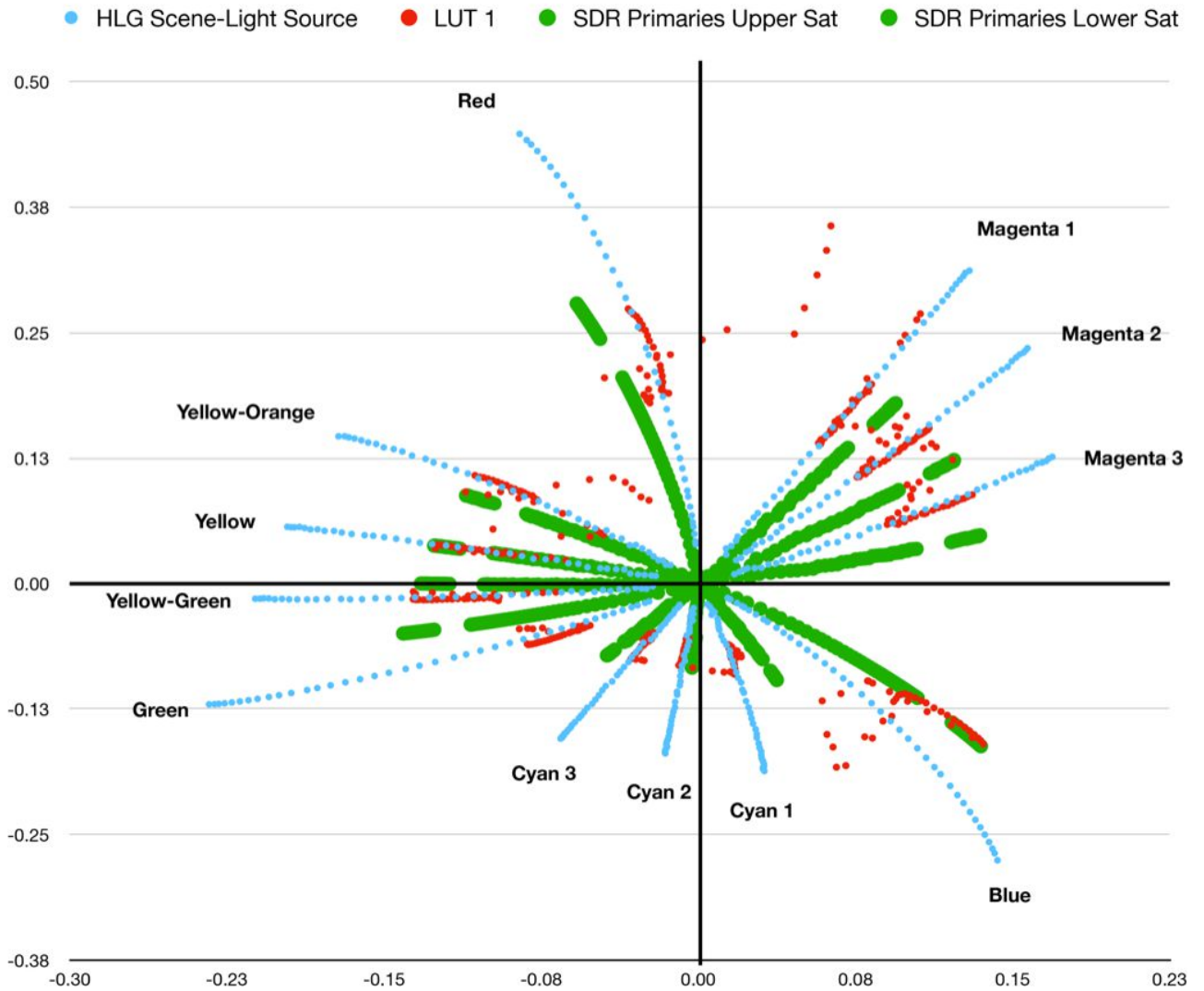
Figure 19 LUT 1 Conversion from HLG to SDR
