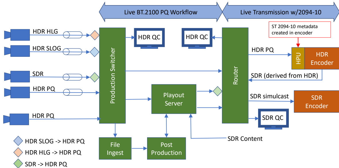
Figure 34 HDR broadcast production facility with BT.2100 PQ workflow-transition phase
